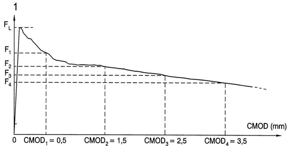
Typical Load deformation Diagram
